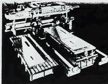
Described in column 1 below, this Kearney and Trecker skin mill is one of the largest machine tools ever to be bought by an aircraft company. The work table is 28ft by 9ft, and a further indication of scale is provided by the operator.
