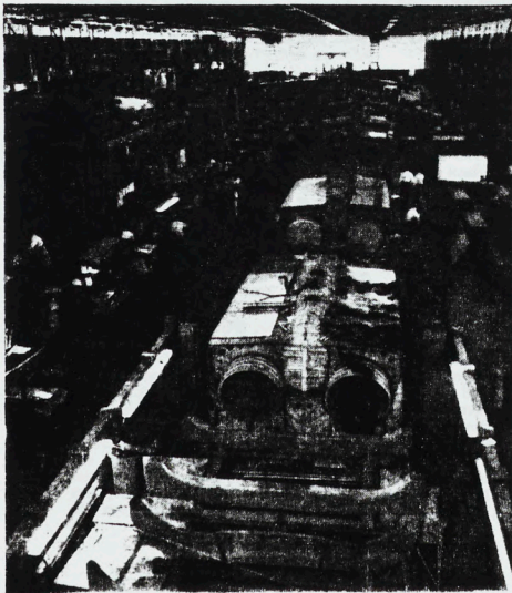
A recent view of Bay 1 at Malton, showing (front to rear): the final "marry-up" jig; a row of Mk 1 centre fuselages; a complete Mk 1; and the metal mock-up, by the exit door.
